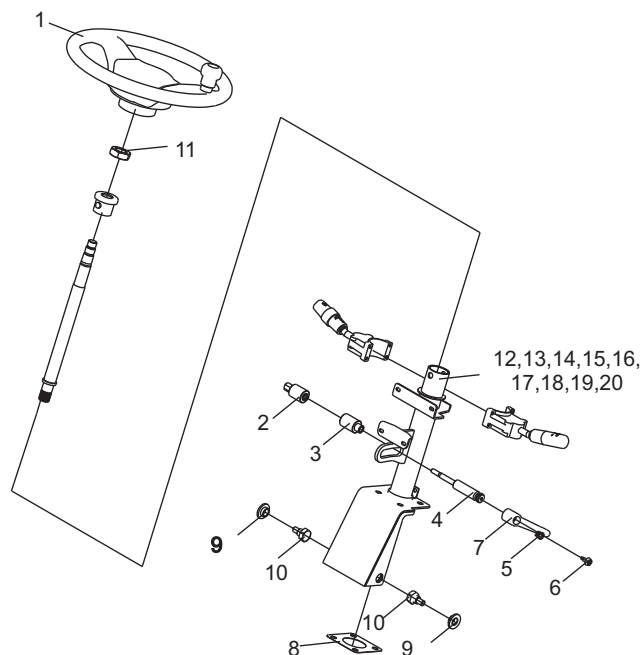
转向操纵总成/ Steering control assy.
