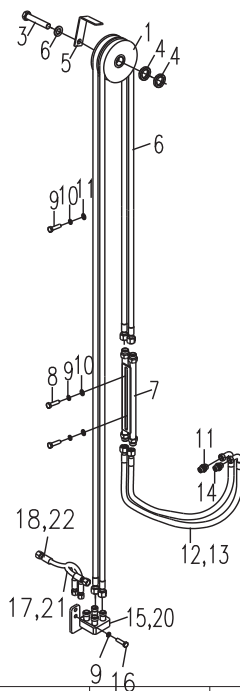
侧移管路(基本型) / Side shifting pipeline (Normal mast)
