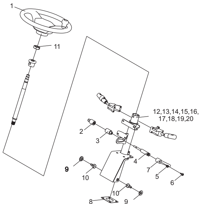
转向操纵总成/ Steering control assy.
