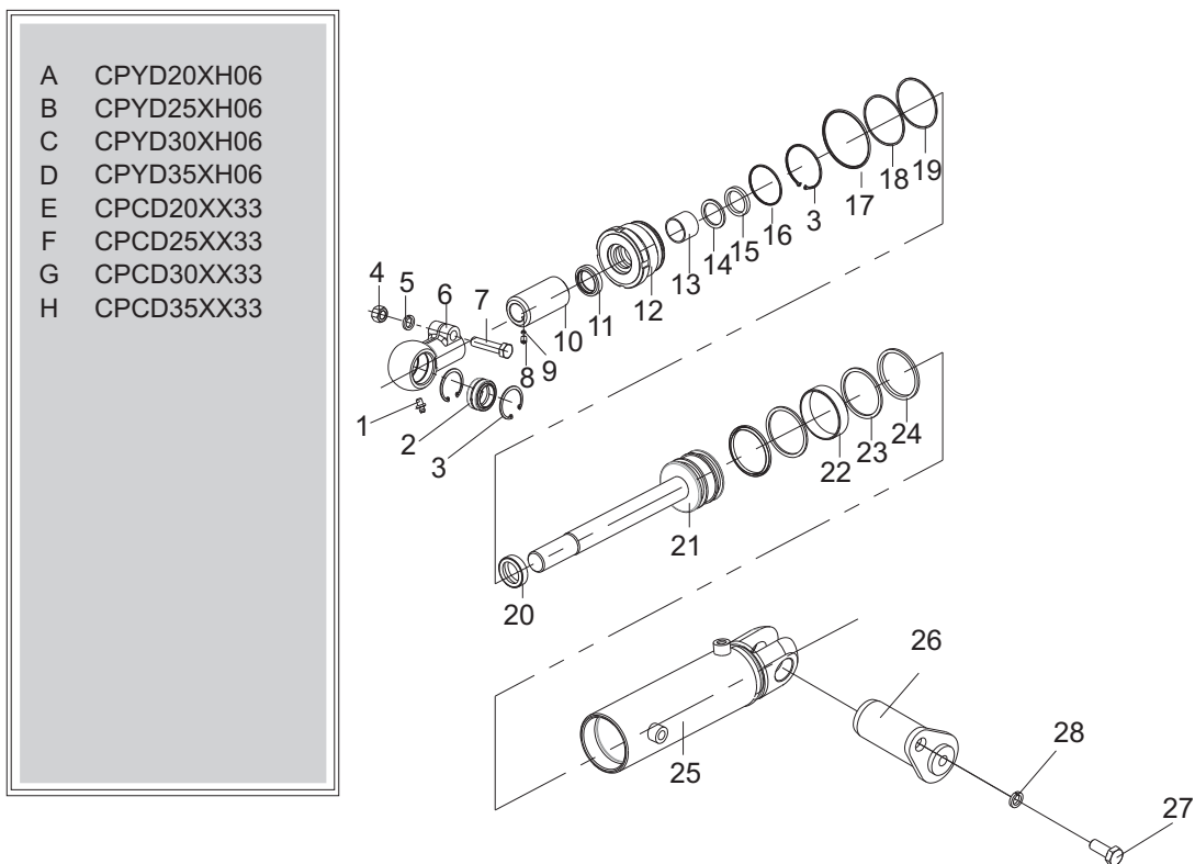
倾斜油缸/Tilt cylinder
