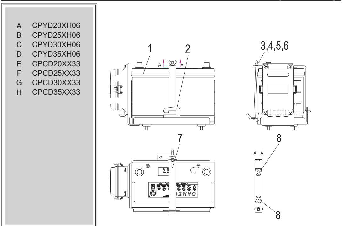
图49/FIG.49 电气元件总成/ Electrical component assy.
