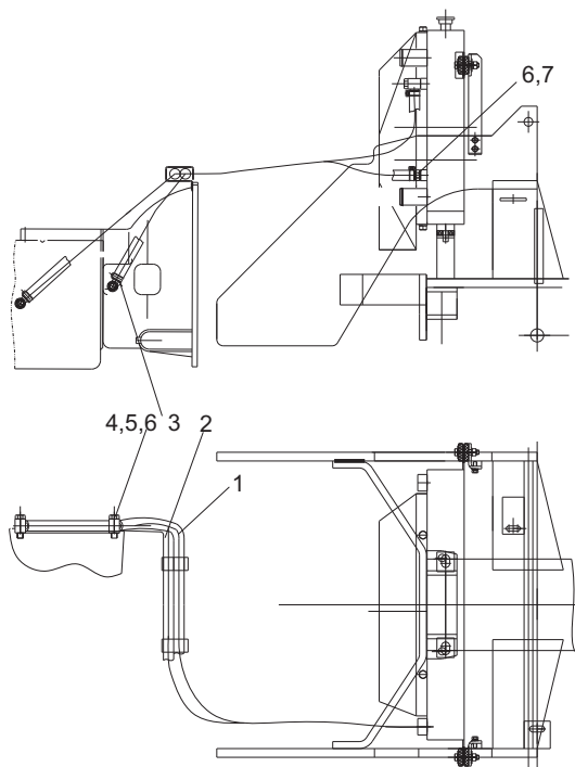
油冷却管路总成/ Oil cooling pipe assembly
