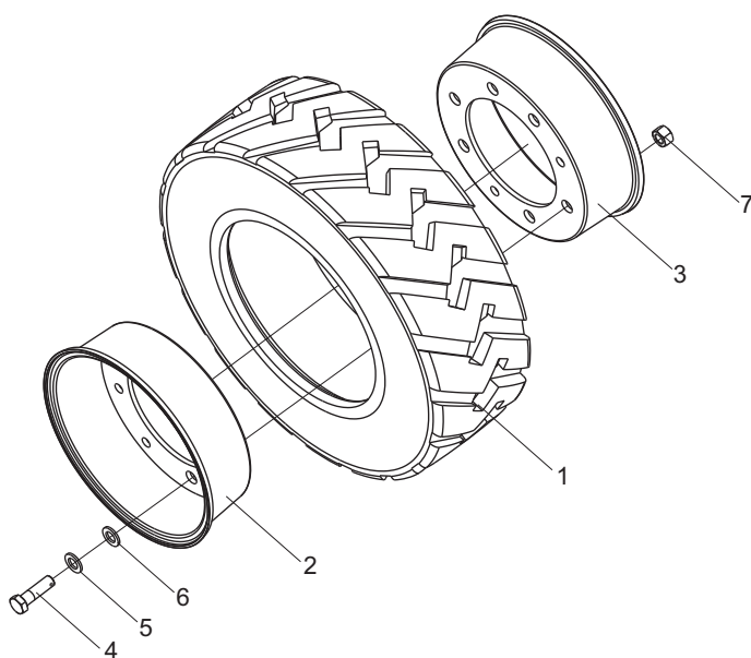
转向轮/Steering wheel
