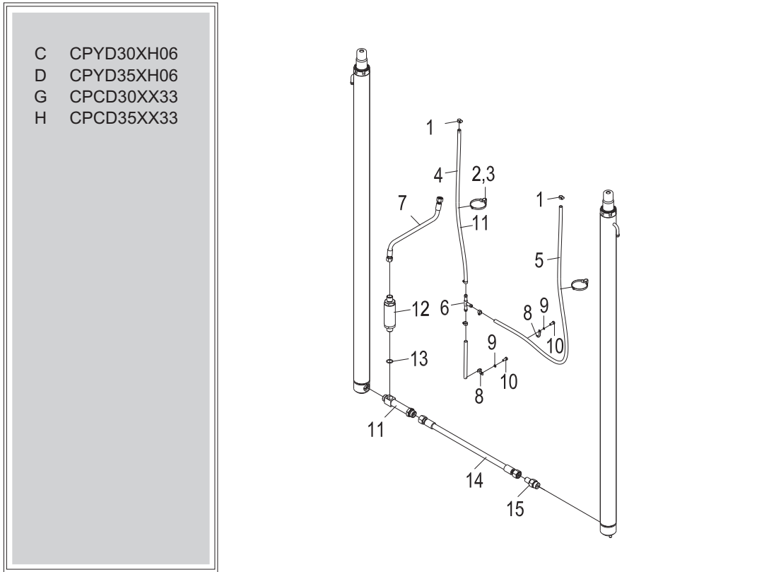
图40/FIG.40 起升管路(基本型) / Lift pipeline (normal mast)
