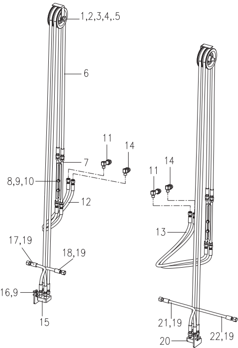
侧移管路(基本型) / Side shifting pipeline (Normal mast)
