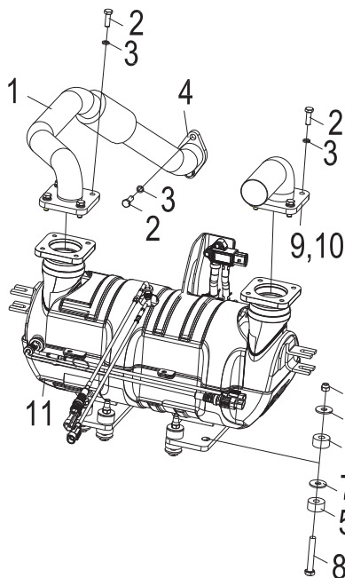
图9/FIG.9 后处理总成/After-treatment assy.
