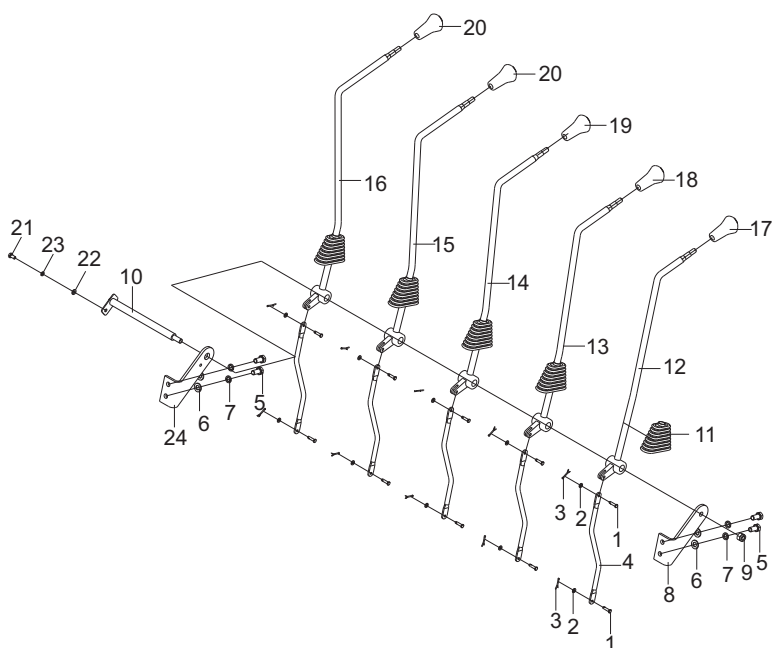
多路阀操纵(五联)/ Multi-way valve control (Quintuplex)
