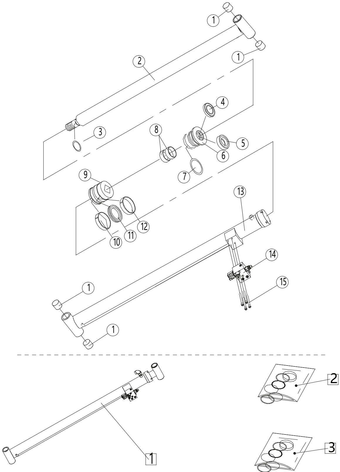
Figure 18 Cylinder (SC12H/SC14H/SC12E/SC14E)
