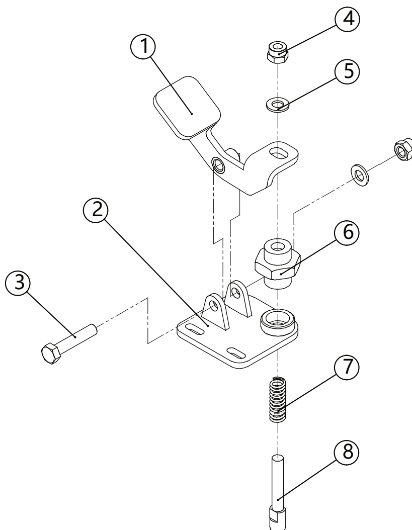
Figure 16.1 Verrouillage de pédale (SC10H/SC12H/SC14H/SC10E/SC12E/SC14E)
