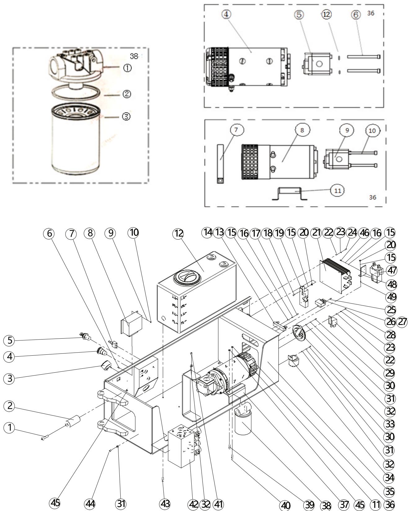
Figure 2.1: Assemblage de la boîte de la station de pompe (SC10H/SC12H/SC14H/SC08HN/SC10HN)
