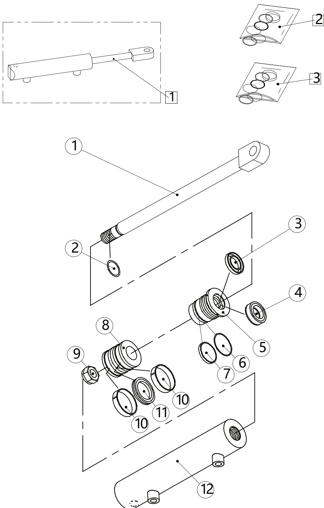
Figure 21 Vérin de direction
