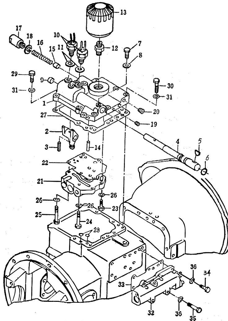
Cover, Control valve, Inching Valve
