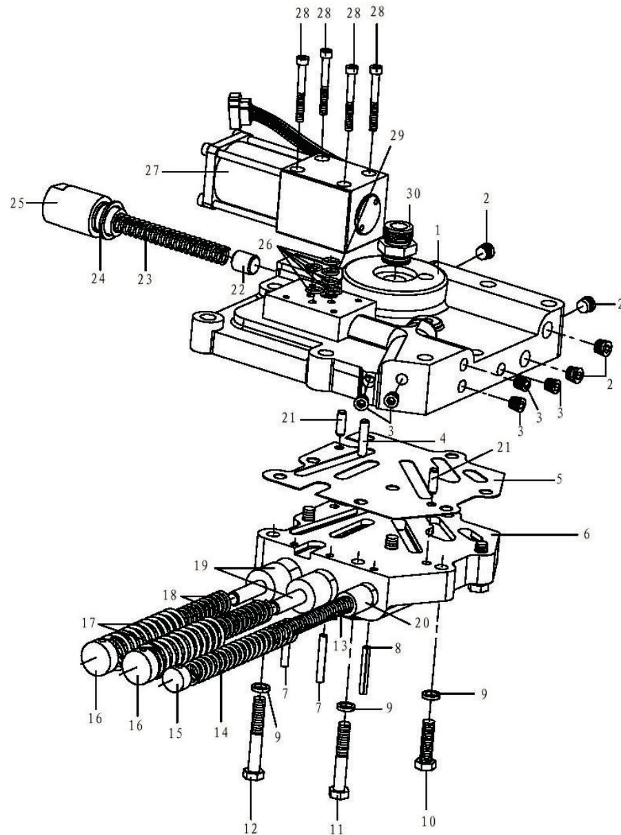
DCCT5 Control valve
