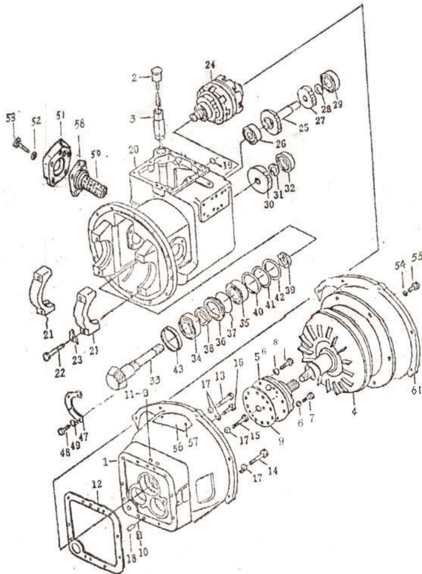
JCMFVD30TXD Gear Box
