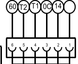
ELECTRONIC REGULATOR PLUG
