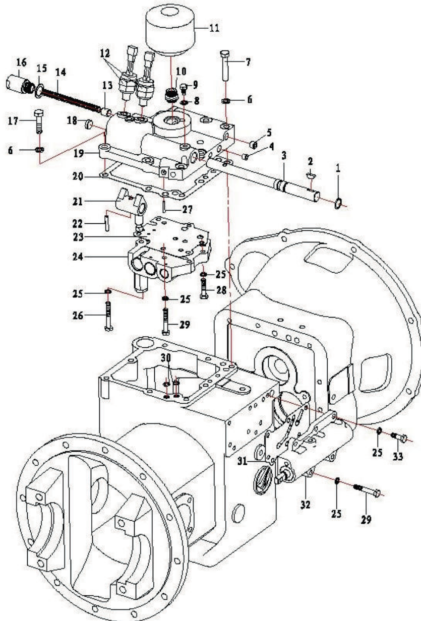
Cover, Control valve, Inching Valve
